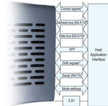
Block diagram
